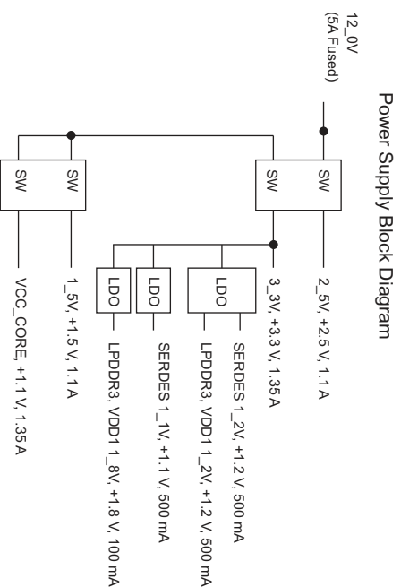
Figure 2. Power Distribution Scheme (See Appendix B, "Power Supplies" sheet)
