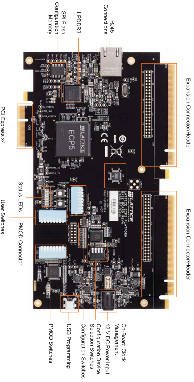
Figure 1. ECP5 PCI Express Board, Top Side
