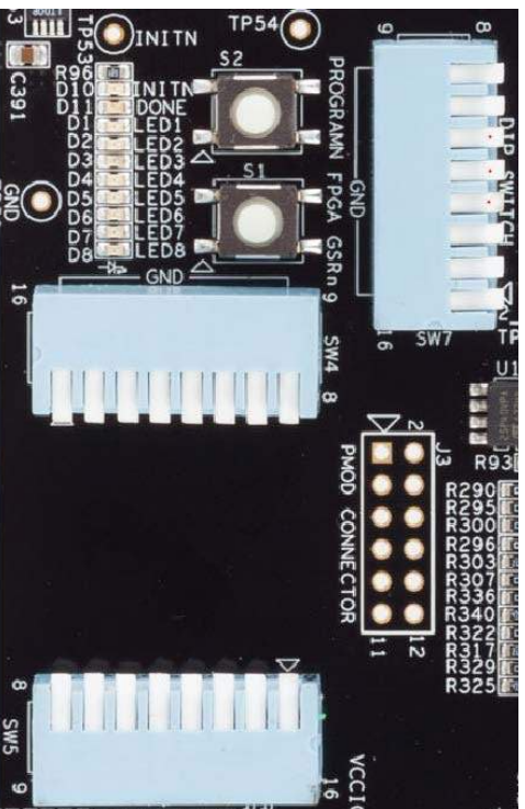
Figure 8. ECP5 PCI Express Board LEDs and Switches
