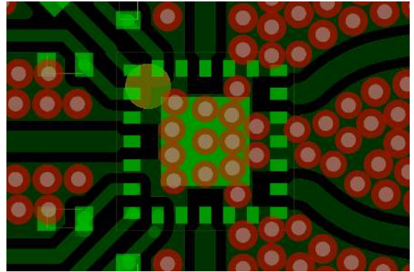
Figure 28. PCB Routings
