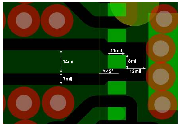
Figure 29. Recommended RF Pin Transitions
