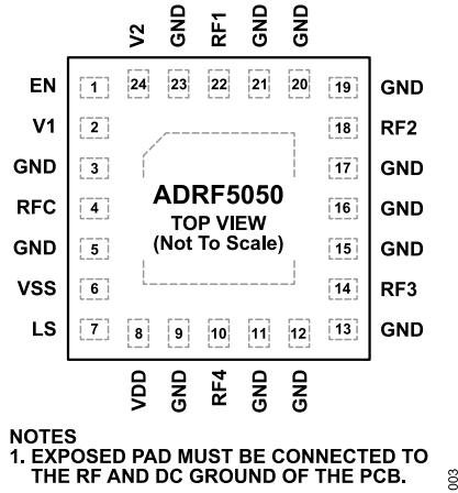
Figure 3. Pin Configuration (Top View)
