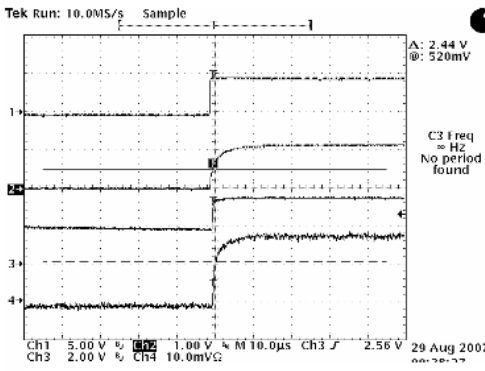
Zoom of the startup Channel 1 Enable; Channel 2 ISET pin; Channel 3 VLED; Channel 4 ILED 20ma/Div
