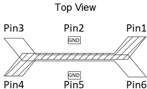
5dB Coupler Pin Configuration
