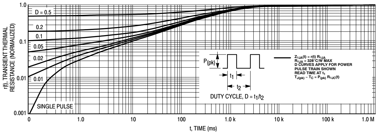
Figure 11. Thermal Response
