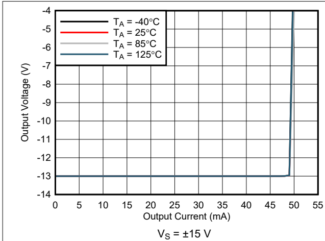
Figure 6-19. Output Voltage Swing vs Output Sinking Current
