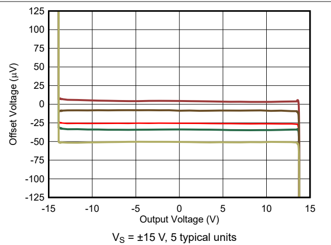
Figure 6-12. Offset Voltage vs Output Voltage
