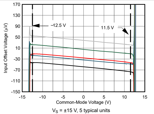
Figure 6-10. Offset Voltage vs Common-Mode Voltage
