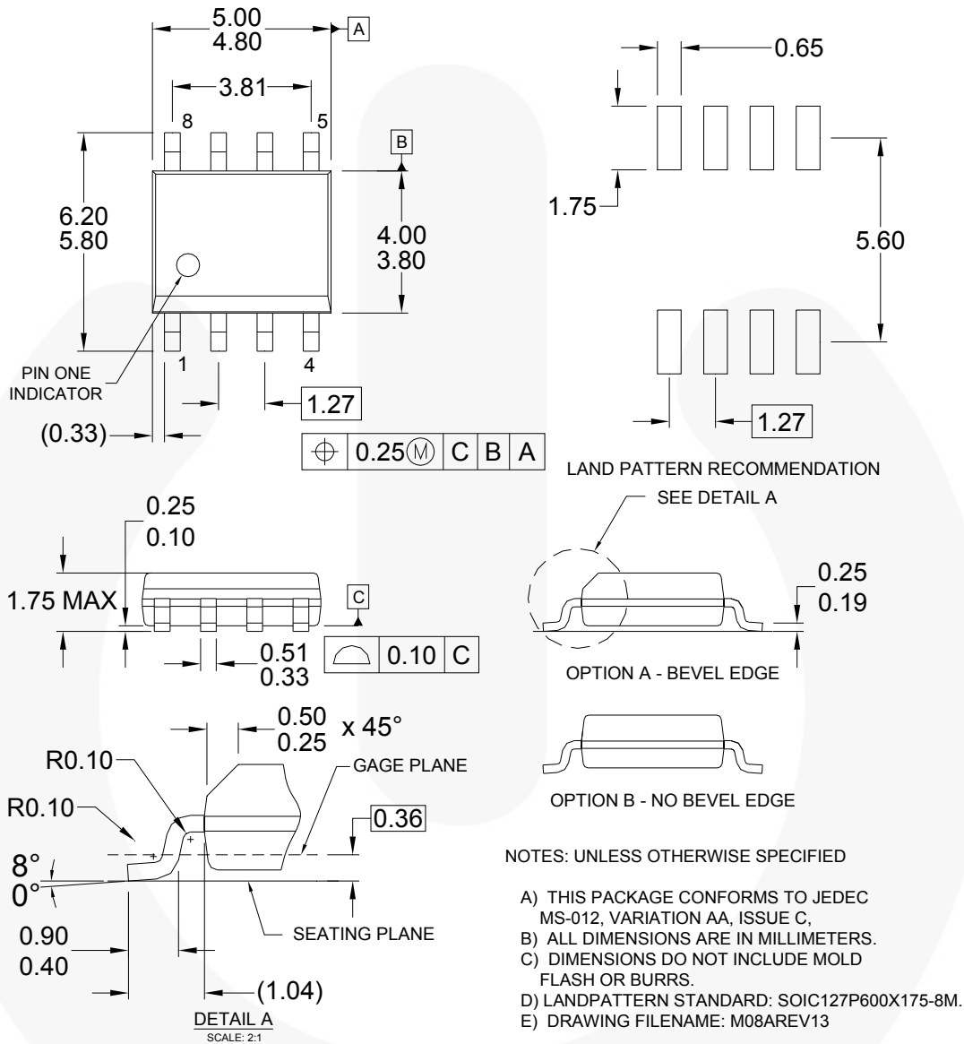
Figure 21. 8-Lead, Small Outline Integrated Circuit (SOIC)
