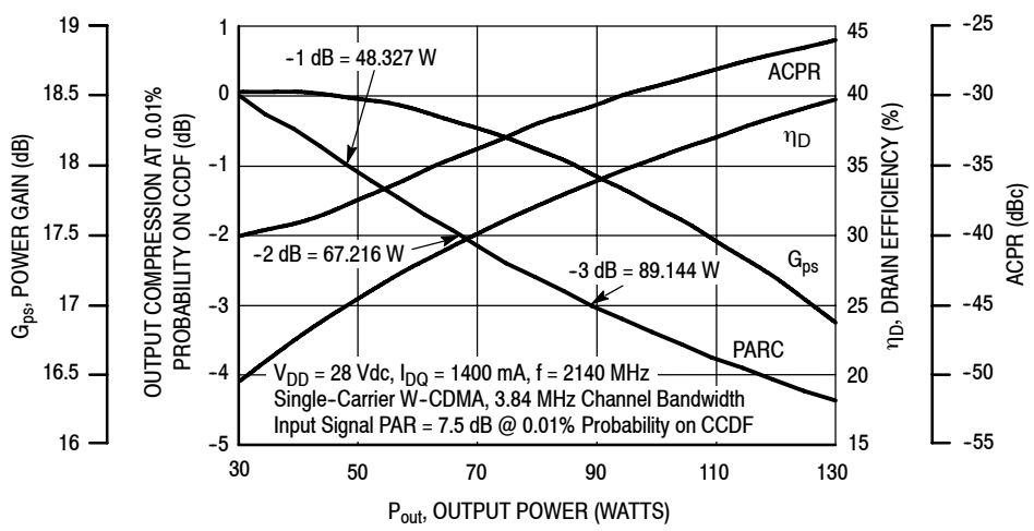
Figure 8. Output Peak-to-Average Ratio Compression (PARC) versus Output Power
