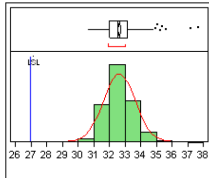
Figure 4. OIP3 Distribution@60mA.
