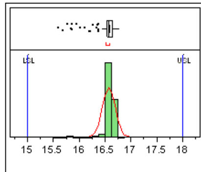
Figure 2. Gain Distribution@60mA.
