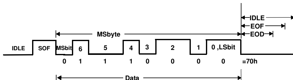
Figure 20. C2Slb Timing Diagram
