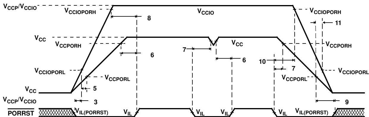
Figure 8. PORRST Timing Diagram
