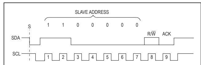
Figure 1. MAX2112 Slave Address Byte with ADDR Pin Connected to Ground
