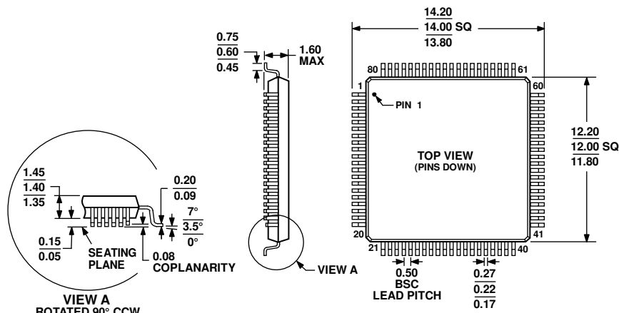
Figure 8. 80-Lead Low Profile Quad Flat Package [LQFP] (ST-80-1)
