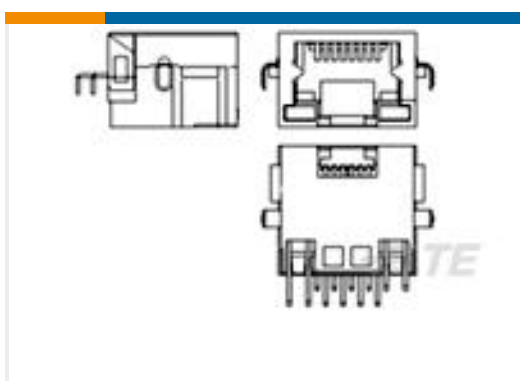
TE Part #2041307-1 RJ45, Shielded, Offset, DIP, 6u", H=8.2
