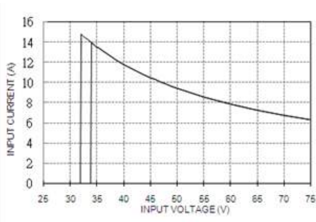
Figure 3: Full load input characteristics at room temperature.
