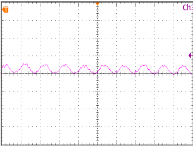
Figure 12: Input reflected ripple current, i_s , through a 12\mu\text{H} source inductor at nominal input voltage and max load current (25mA/div, 4µs/div).
