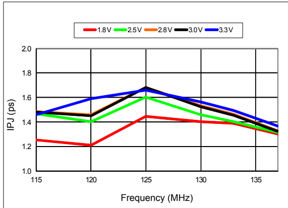
Figure 14. RMS Integrated Phase Jitter Random (12 kHz to 20 MHz) vs Frequency [11]
