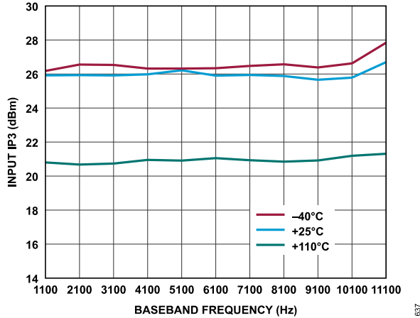
Figure 296. Receiver Input IP3 vs. Baseband Frequency, ADC = High Performance, f_1 = Baseband Frequency + 1 MHz, f_2 = Baseband Frequency + 2 MHz, Gain Index = 255, First-Order TIA with f_{1dB} = 4 MHz, P_{OUT} = -13.6 dBFS at -40°C and +25°C, P_{OUT} = -16.6 dBFS at +110°C
