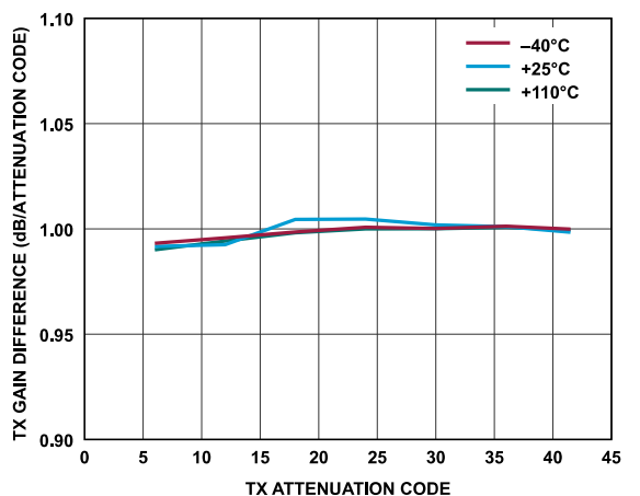
Figure 31. Transmitter Attenuation Delta (Error) vs. Transmitter Attenuation Code, Baseband Frequency = 18 MHz, Backoff = 0.2 dBFS
