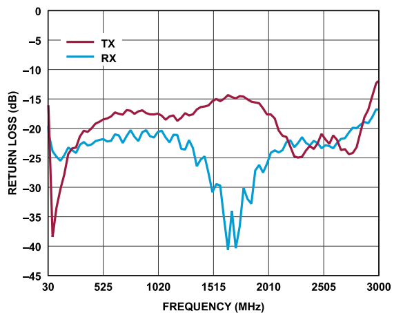
Figure 29. Receiver and Transmitter Return Loss vs. Frequency (For LO = 30 MHz to 3 GHz)
