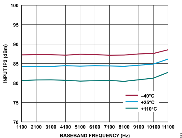
Figure 253. Receiver Input IP2 vs. Baseband Frequency, ADC = Low Power, f_1 = \text{Baseband Frequency} + 1 \text{ MHz} , f_2 = \text{Baseband Frequency} + 2 \text{ MHz} , Gain Index = 255, First-Order TIA with f_{3dB} = 4 \text{ MHz} , P_{OUT} = -11.6 \text{ dBFS}
