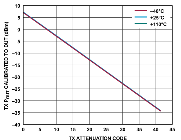
Figure 30. Transmitter Absolute Power vs. Transmitter Attenuation Code, Baseband Frequency = 18 MHz, Backoff = 0.2 dBFS
