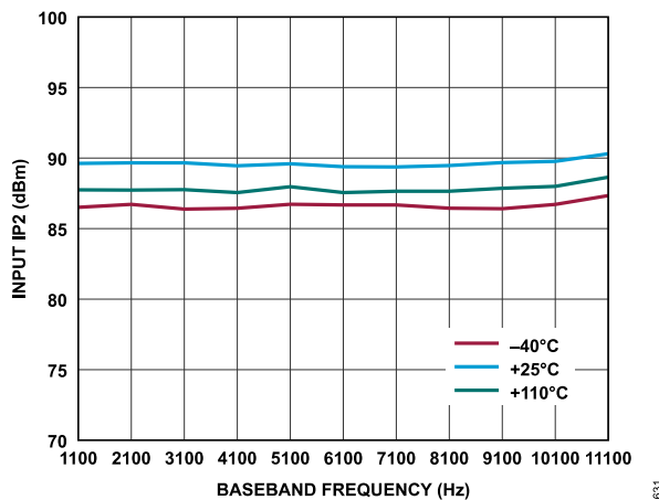
Figure 252. Receiver Input IP2 vs. Baseband Frequency, ADC = High Performance, f_1 = \text{Baseband Frequency} + 1 \text{ MHz} , f_2 = \text{Baseband Frequency} + 2 \text{ MHz} , Gain Index = 255, First-Order TIA with f_{3dB} = 4 \text{ MHz} , P_{OUT} = -11.6 \text{ dBFS}
