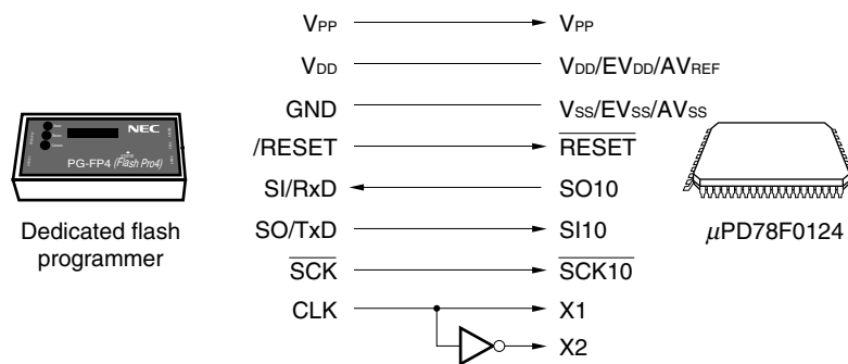
Figure 25-8. Communication with Dedicated Flash Programmer (CSI10)
