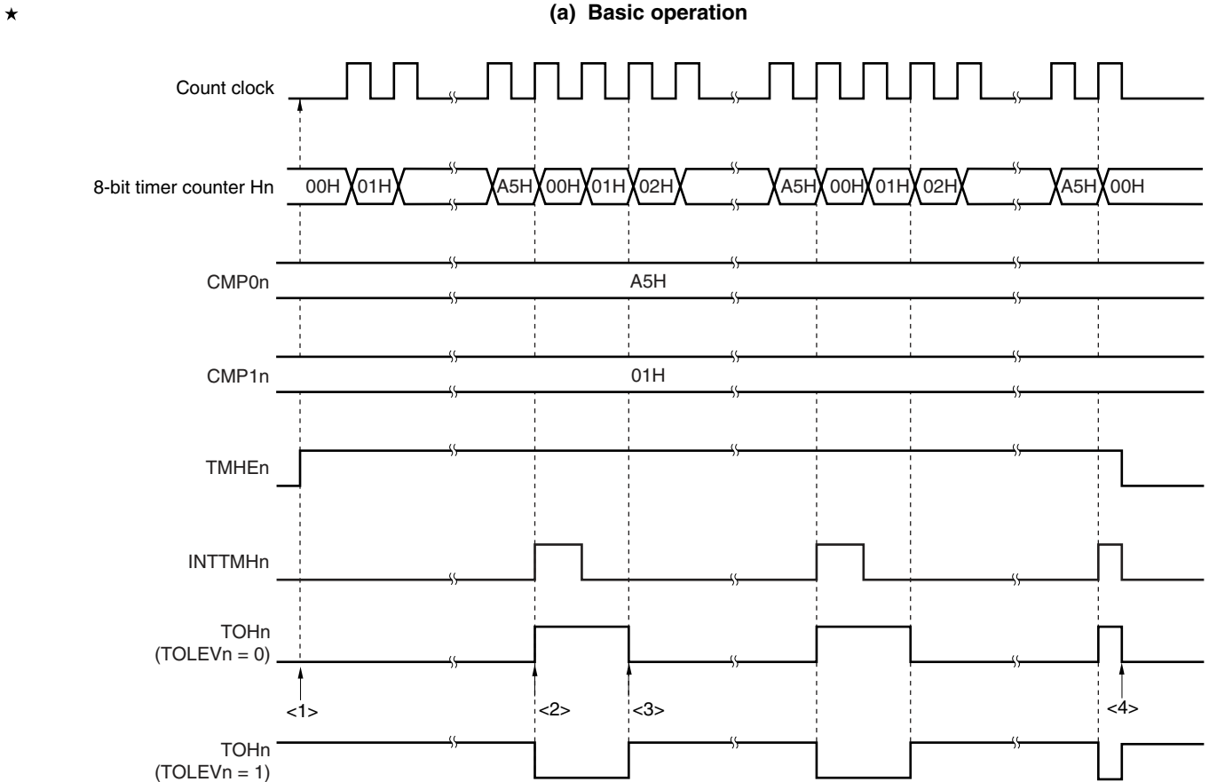
Figure 8-12. Operation Timing in PWM Output Mode (1/4)
