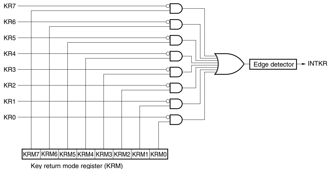
Figure 17-1. Block Diagram of Key Interrupt
