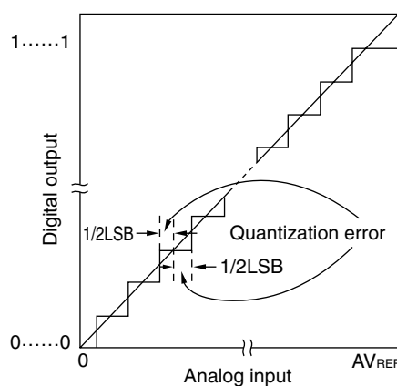
Figure 12-13. Quantization Error
