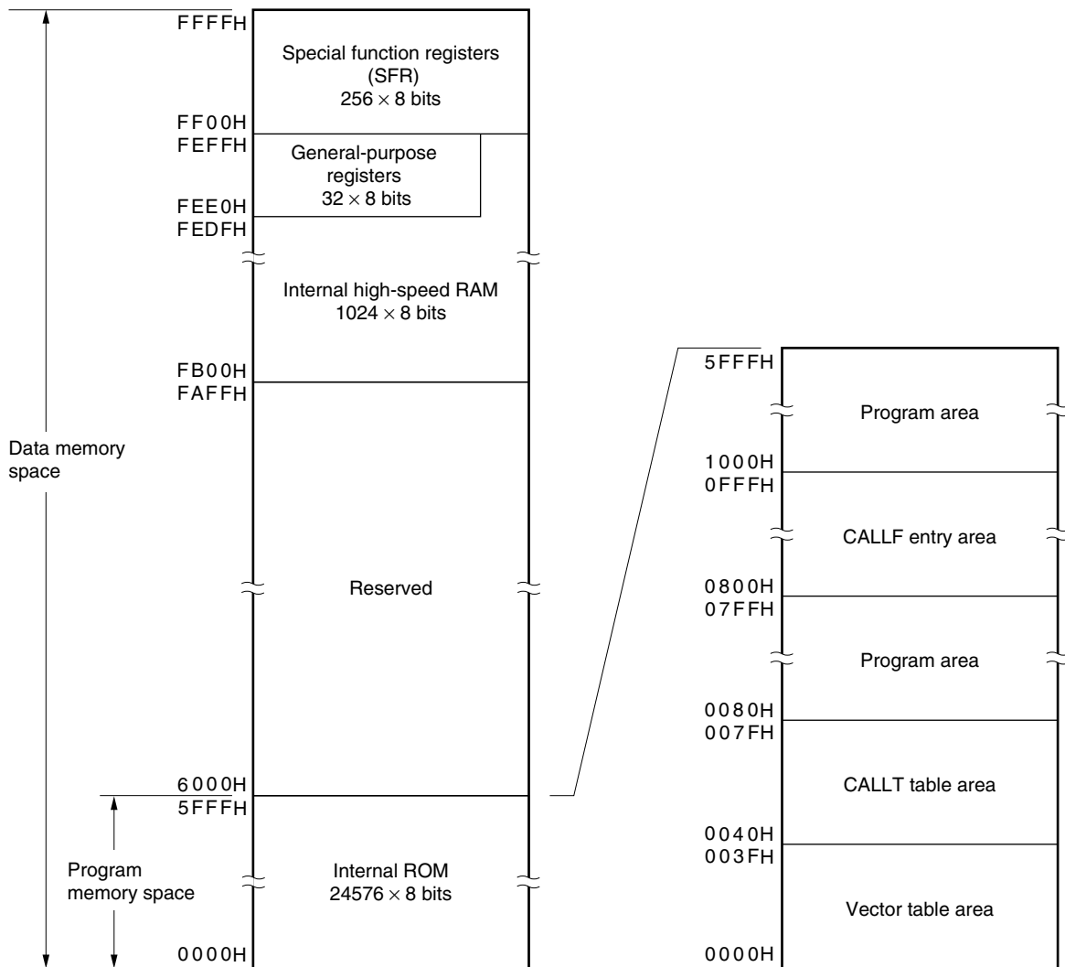
Figure 3-3. Memory Map ( \mu PD780123)
