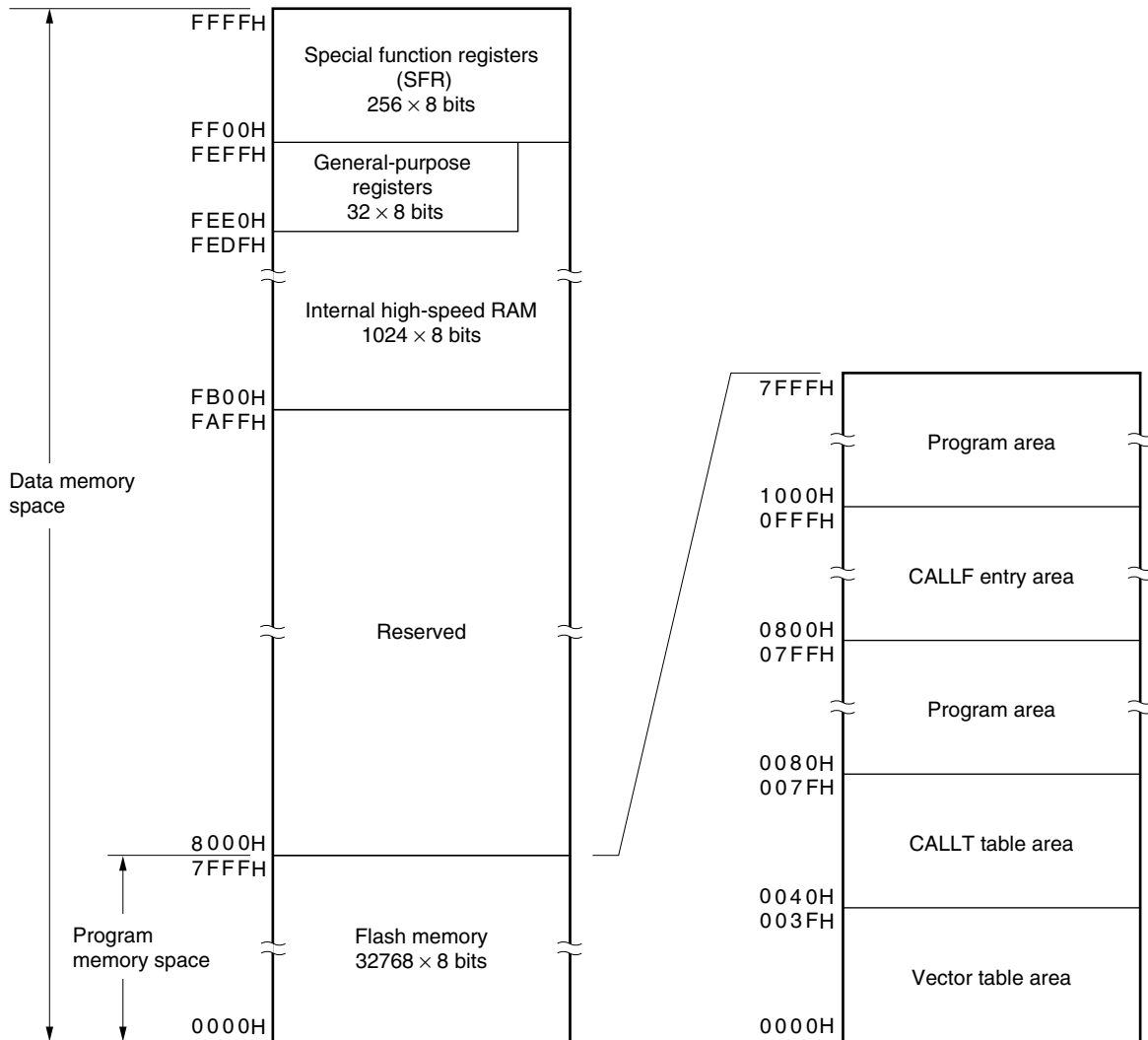
Figure 3-5. Memory Map ( \mu PD78F0124)
