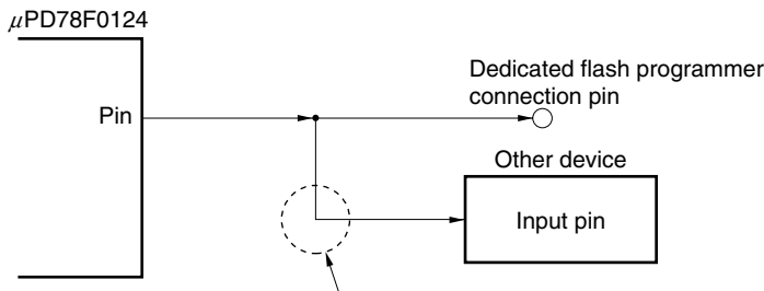
Figure 25-15. Malfunction of Other Device
