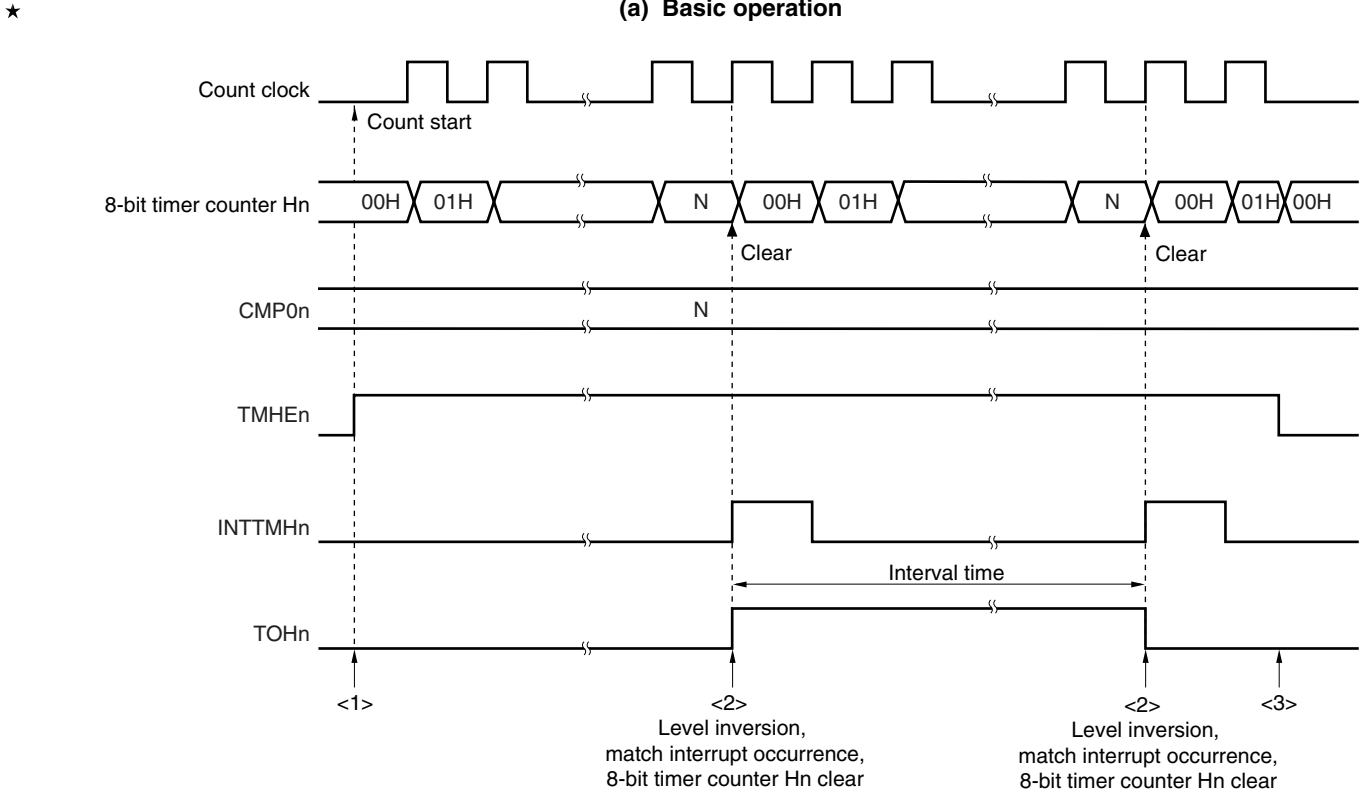
Figure 8-10. Timing of Interval Timer/Square-Wave Output Operation (1/2)
