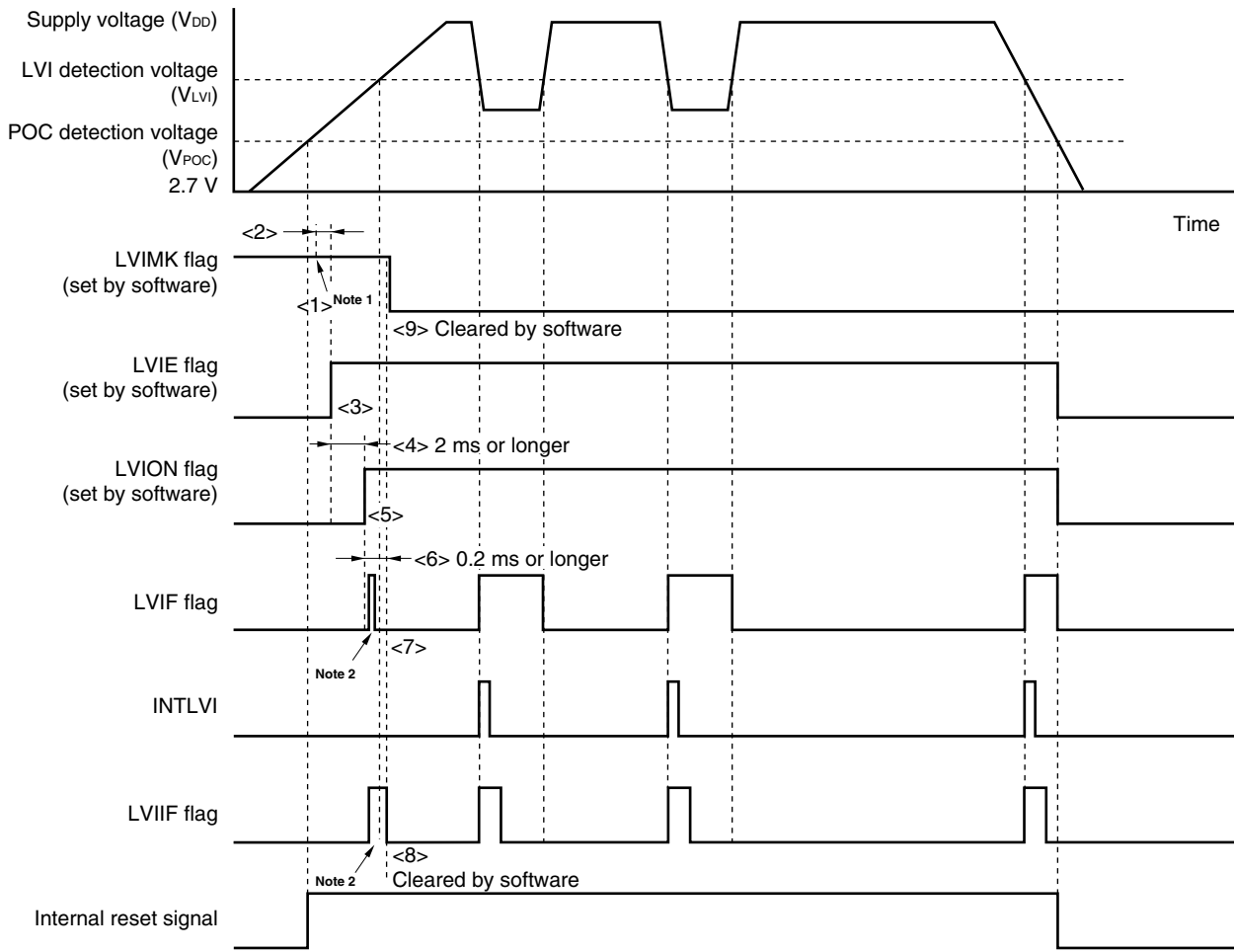
★ Figure 22-5. Timing of Low-Voltage Detector Interrupt Signal Generation
