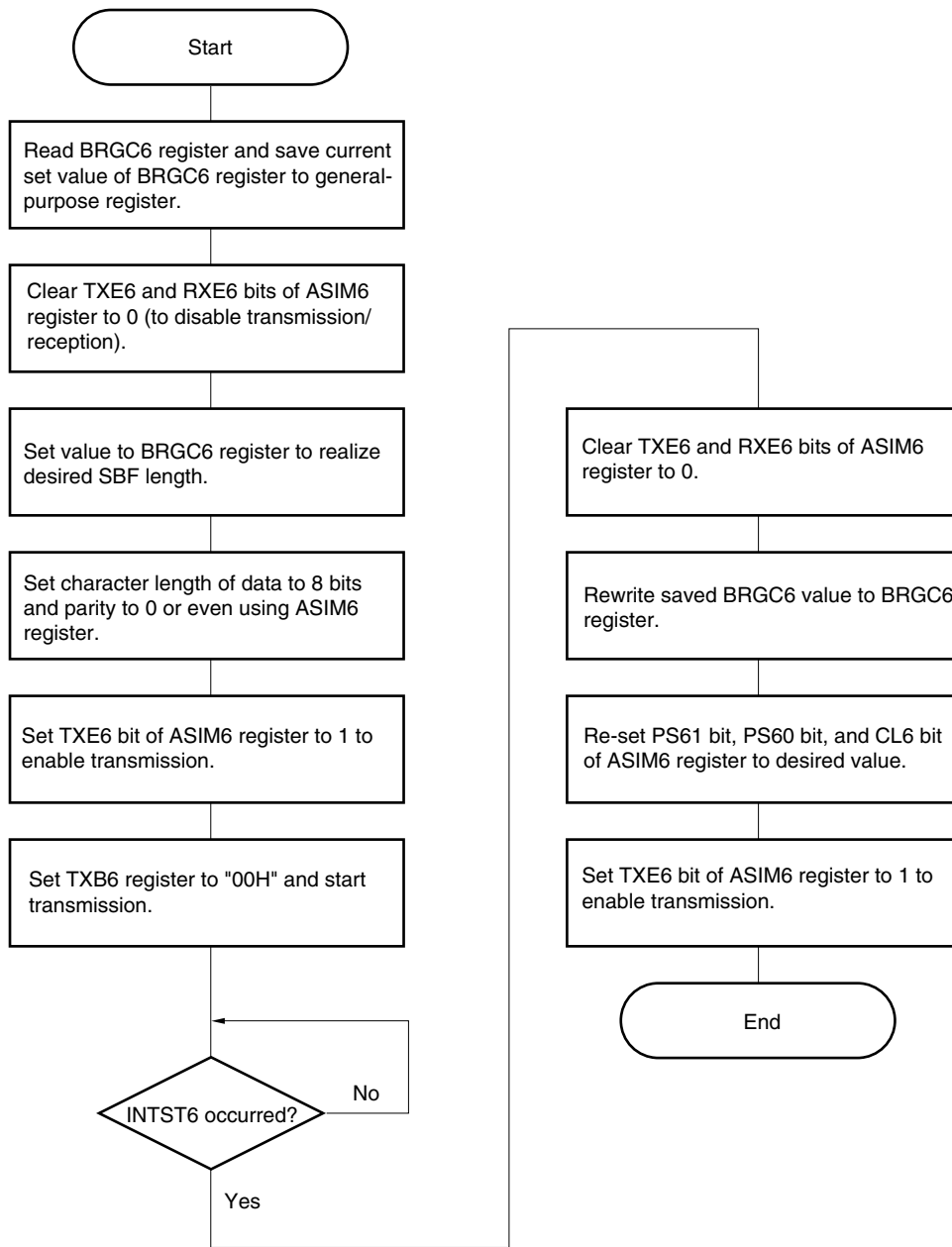
Figure 14-23. SBF Transmission
