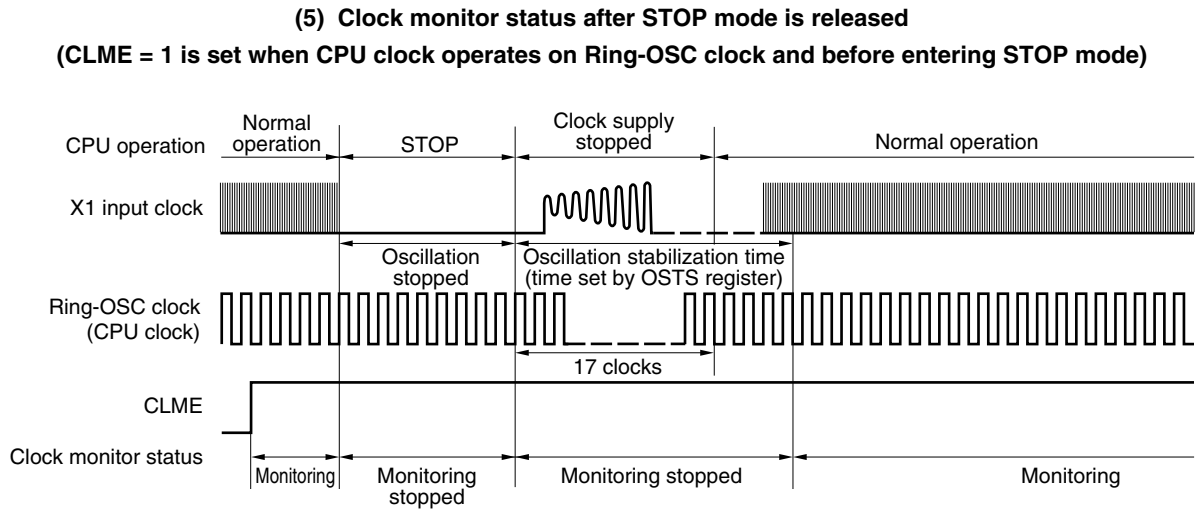
Figure 20-3. Timing of Clock Monitor (3/4)
