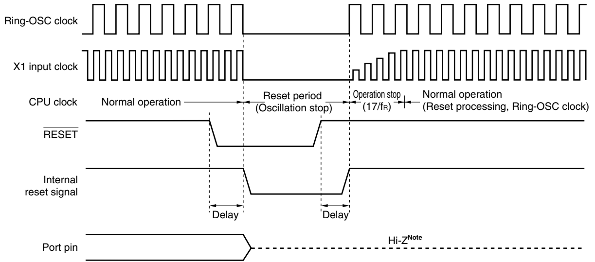
Figure 19-2. Timing of Reset by \overline{\text{RESET}} Input
