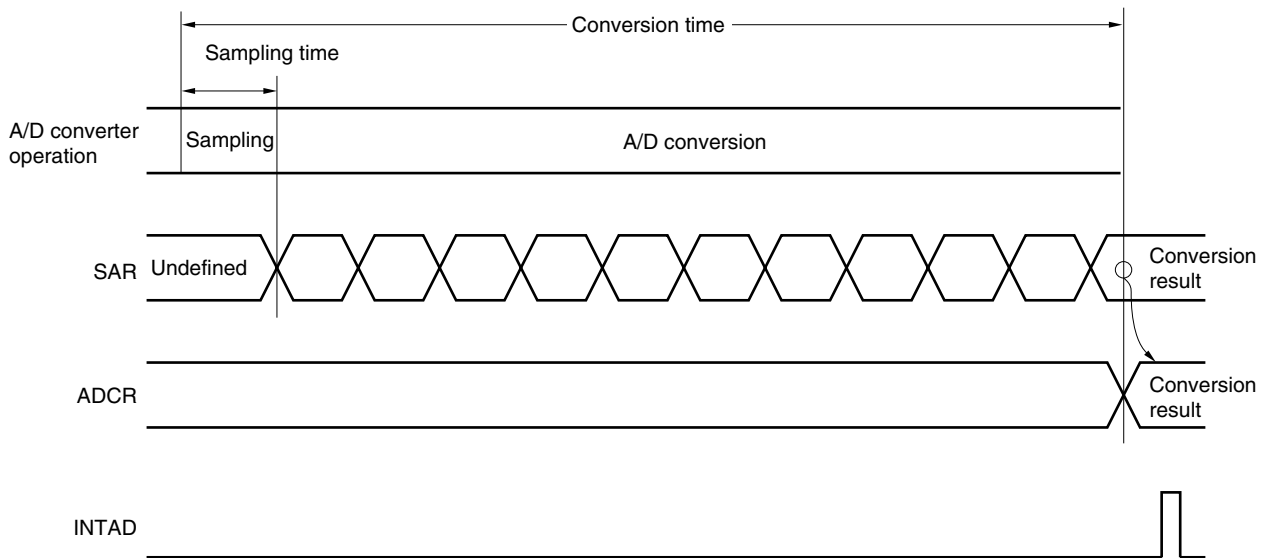
Figure 12-8. Basic Operation of A/D Converter
