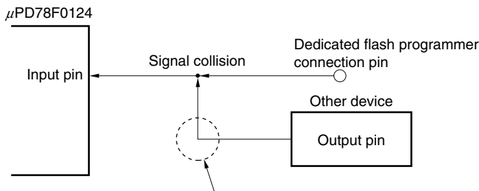
Figure 25-14. Signal Collision (Input Pin of Serial Interface)
