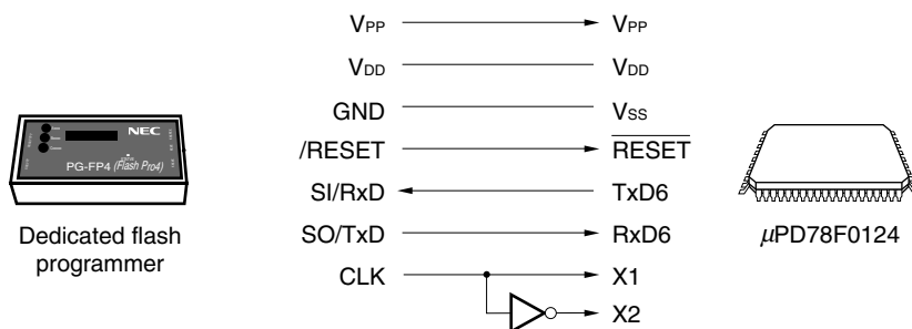
Figure 25-12. Communication with Dedicated Flash Programmer (UART6)
