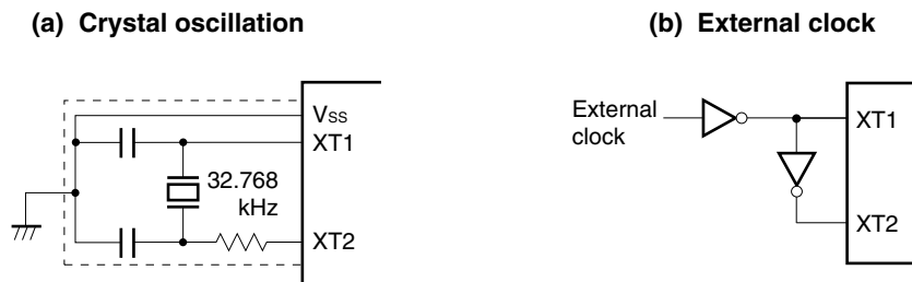
Figure 5-9. Examples of External Circuit of Subsystem Clock Oscillator
