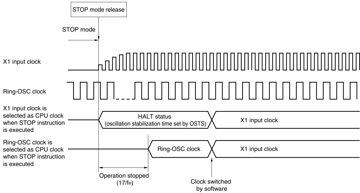
Figure 18-5. Operation Timing When STOP Mode Is Released
