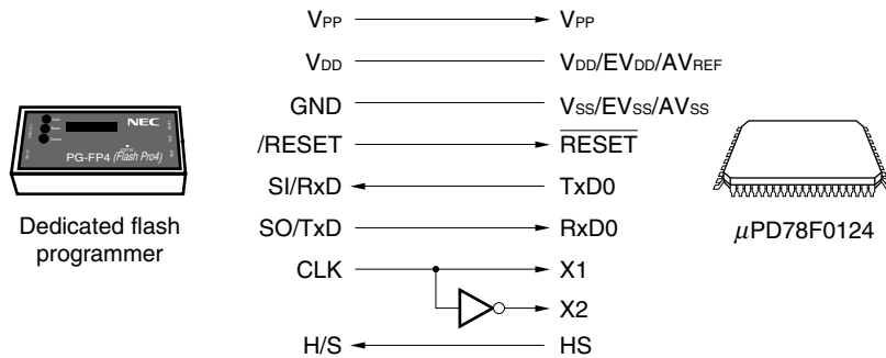
Figure 25-11. Communication with Dedicated Flash Programmer (UART0 + HS)
