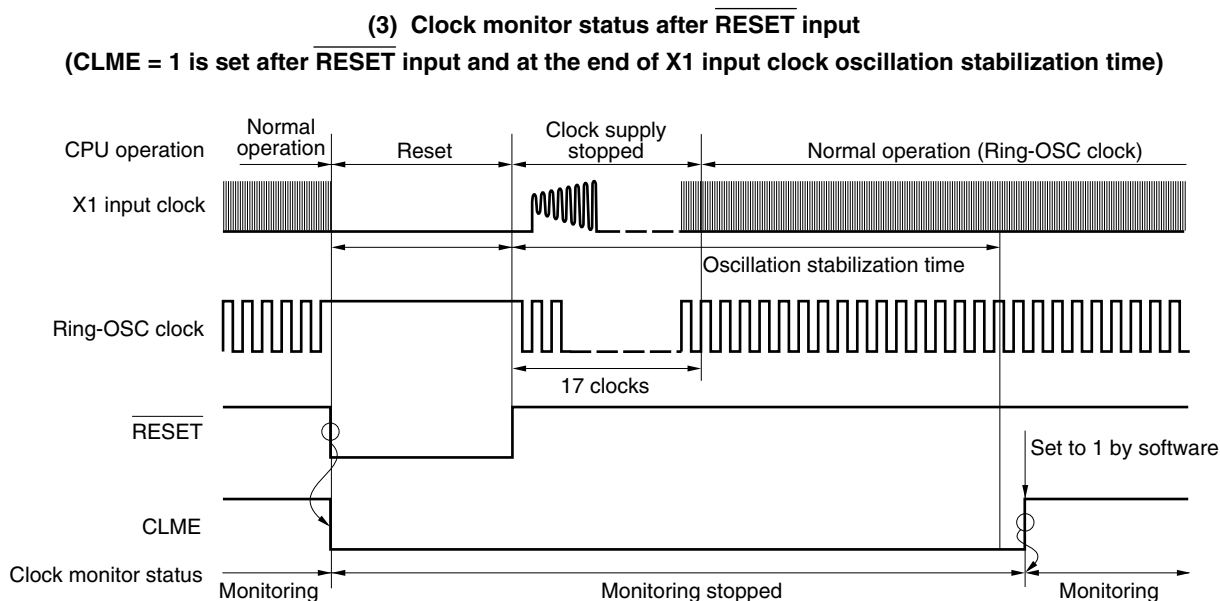
Figure 20-3. Timing of Clock Monitor (2/4)
