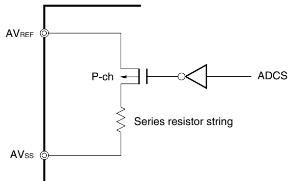
Figure 12-18. Circuit Configuration of Series Resistor String
