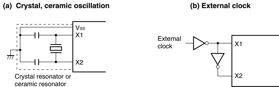
Figure 5-8. Examples of External Circuit of X1 Oscillator
