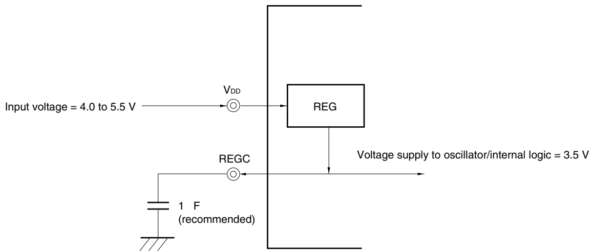
(b) When connecting REGC pin to V SS via a capacitor
