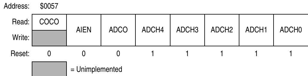
Figure 15-3. ADC Status and Control Register (ADSCR)
