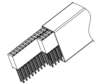
3D View for 52pins After packing
