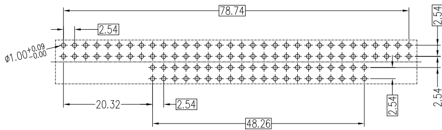
Recommended P.C.B Layout for 52pins (Top Side) (PCB BOARD TOLERANCE±0.05)
