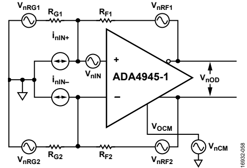
Figure 102. ADA4945-1 Noise Model
