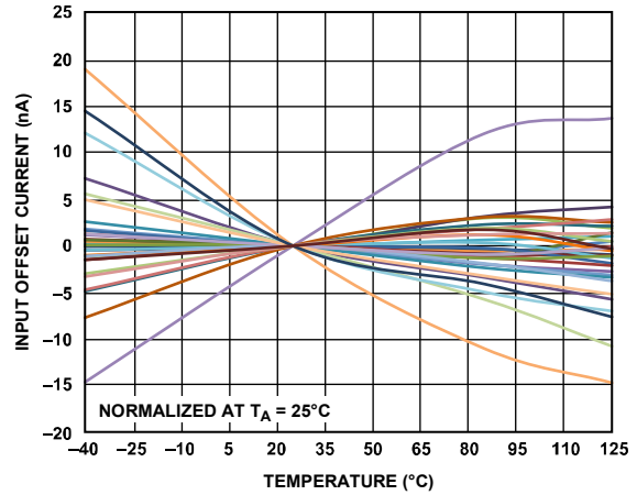
Figure 64. Input Offset Current vs. Temperature for 30 Devices
