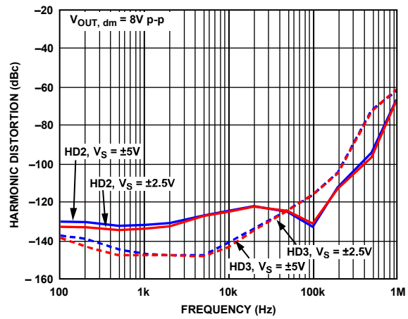
Figure 66. Harmonic Distortion vs. Frequency for Various Supplies
