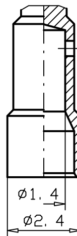
Detail "X" M 10: 1
