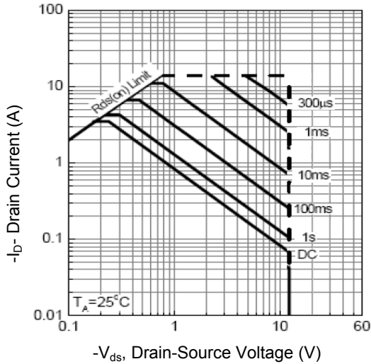
Figure 13. Safe Operation Area
