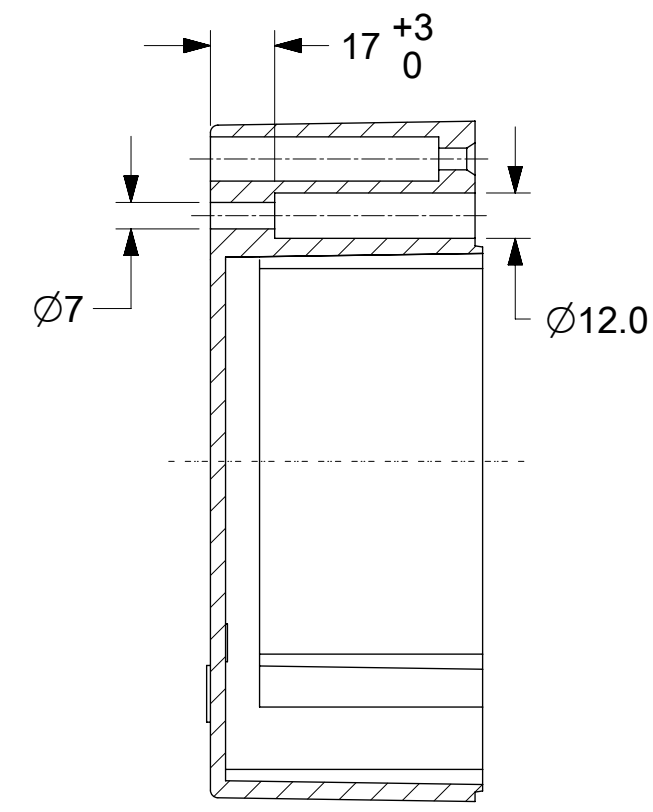
SECTION C-C
