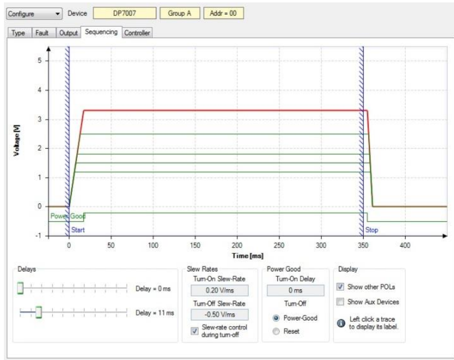
Figure 18. dPOL Configure Sequencing Window
