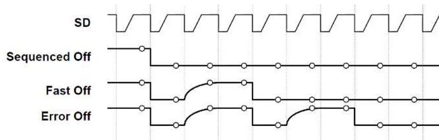
Figure 42. OK Severity Encoding Waveforms
