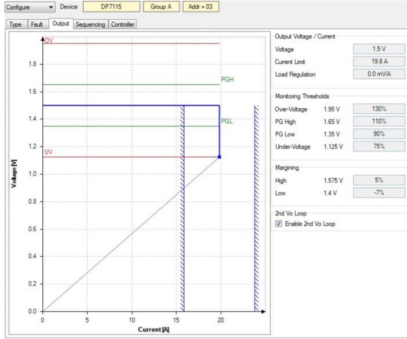
Figure 13. Output Configuration Window
