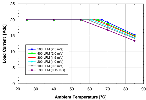
Figure 3. Available output current vs. ambient air temperature and airflow rates for converter DP8120G mounted horizontally with air flowing from input to output, MOSFET temperature 120\text{ }^{\circ}\text{C} , V_{in} = 12\text{ V} , V_{out} = 5\text{ V} , and F_{sw} = 500\text{ KHz}
