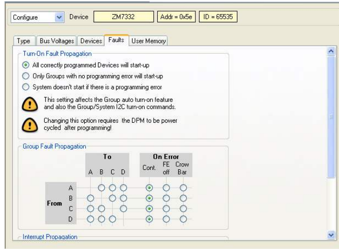
Figure 36. DPM Configure Faults Window
