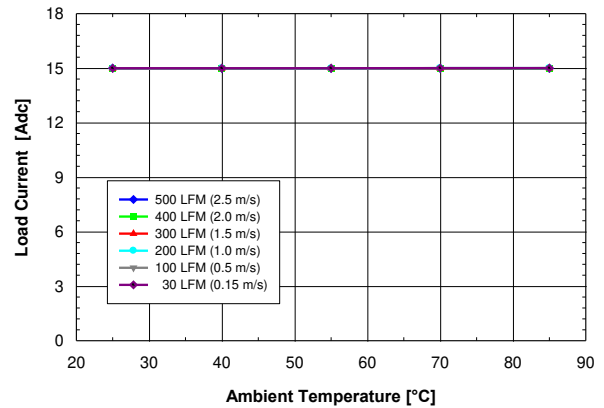
Figure 4. Available output current vs. ambient air temperature and airflow rates for converter DP8120G mounted horizontally with air flowing from input to output, MOSFET temperature 120\text{ }^{\circ}\text{C} , V_{in} = 12\text{ V} , V_{out} = 5\text{ V} , and F_{sw} = 1\text{ MHz}
