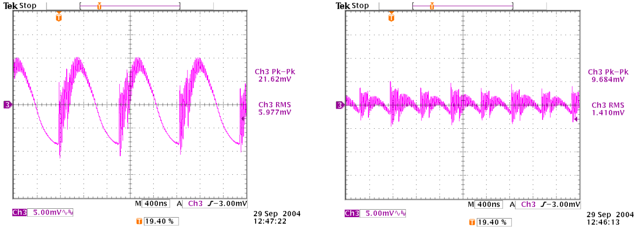
Figure 48. Output Voltage Noise, Full Load, 180° Interleave
