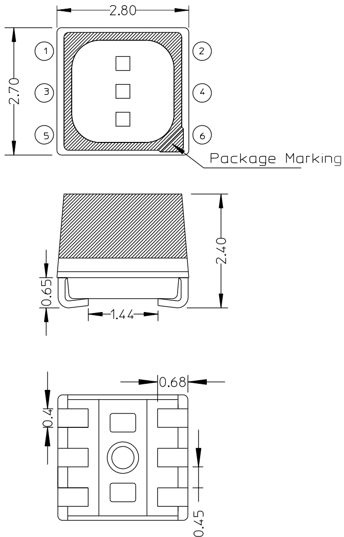
Figure 1: Package Drawing
