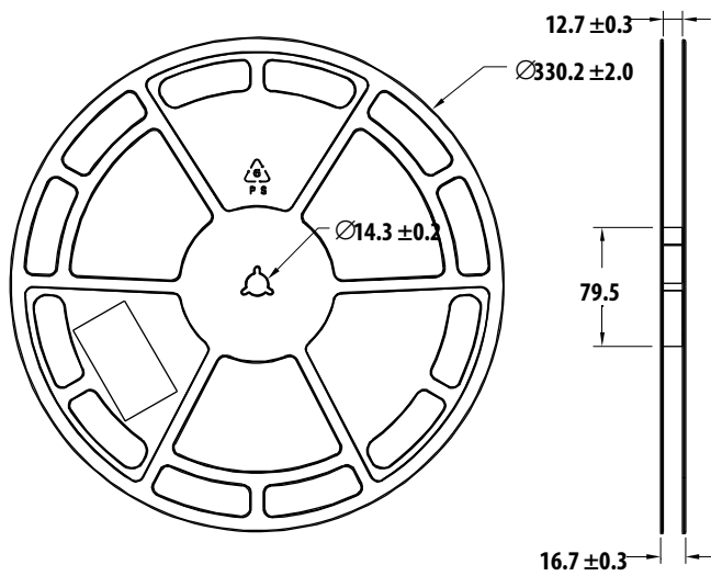
Figure 14: Reel Dimensions
