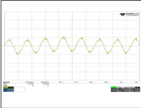
Figure 1: AVD50B-48S3V3 Input Reflected Ripple Current Waveform Ch 1: lin (2µs/div, 10mA/div)
