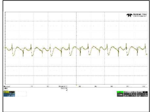
Figure 2: AVD50B-48S3V3 Ripple and Noise Measurement Ch 1: Vo (2µs/div, 20mV/div)
