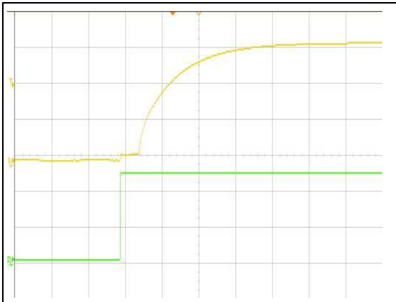
Figure 3: AVD50B-48S3V3 Turn On Characteristic (10ms/div) Ch 1: Vo (1V/div) Ch 2: Vin (20V/div)
