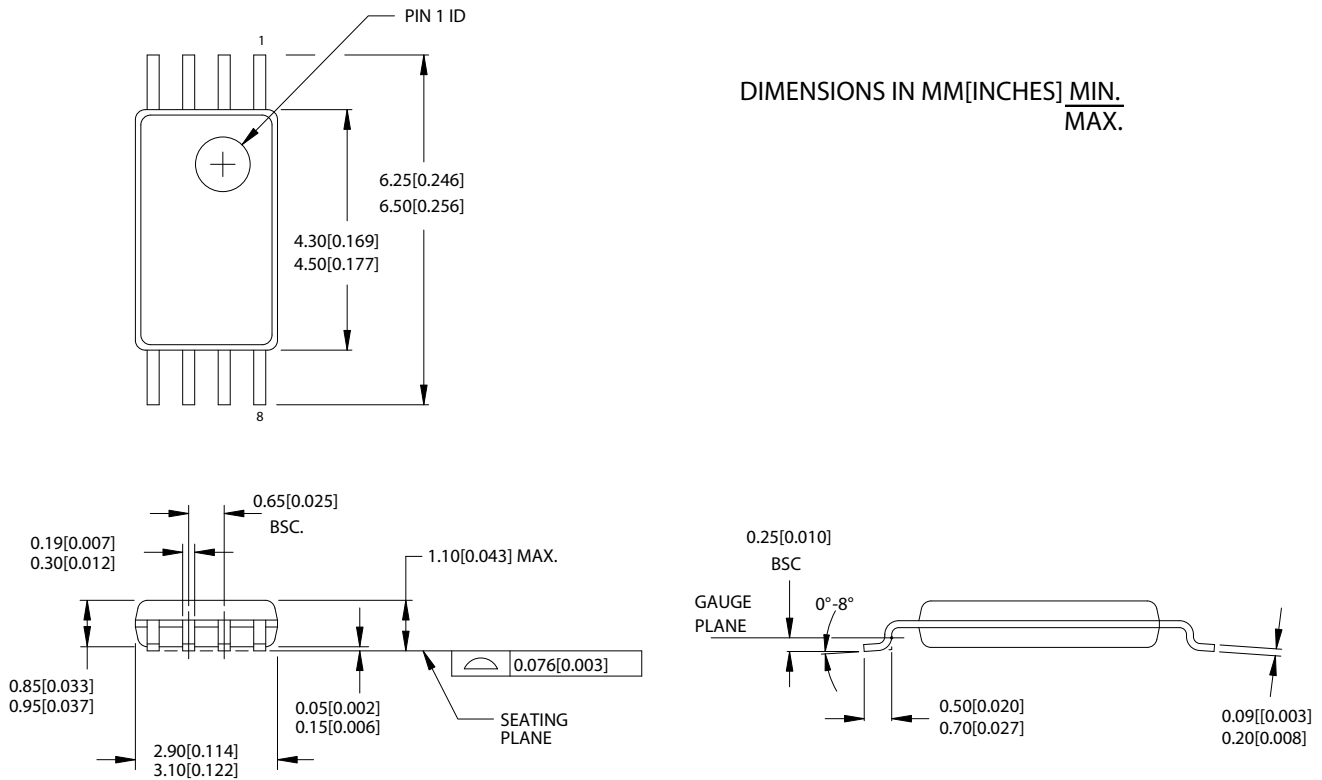
Figure 7. 8-Pin Thin Shrunken Small Outline Package (4.40 mm Body) Z8
