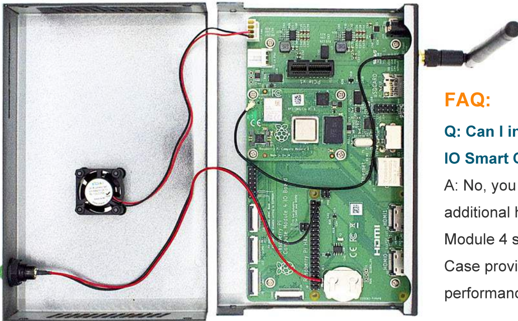
Internal structure after the Compute Module 4 & IO Board installed
