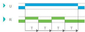
Function Di - Symmetrical flashing (ON Start)
