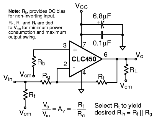
Figure 2: Inverting Configuration
