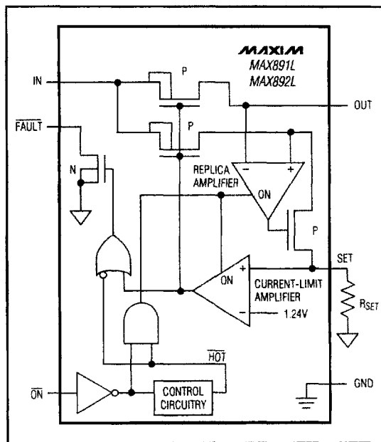
Figure 1. Functional Diagram
