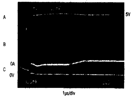
CURRENT-LIMIT RESPONSE (MAX891L, R_L = 0.5\Omega )
