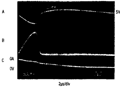
CURRENT-LIMIT RESPONSE (MAX891L, R_L = 0.8\Omega )
