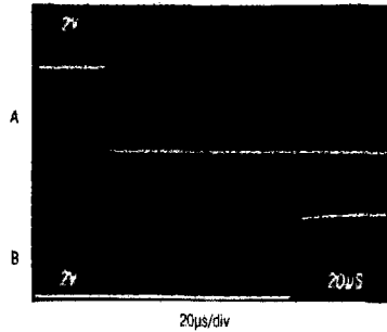
SWITCH TURN-ON TIME
