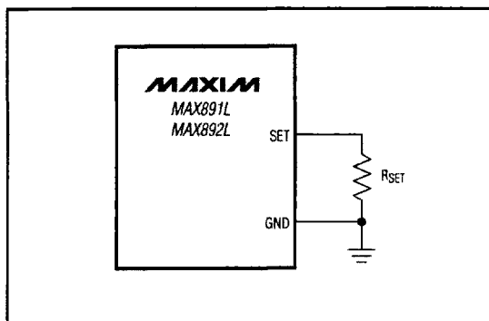
Figure 2. Setting the Current Limit
