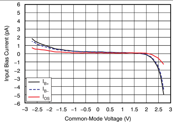
Figure 4. Input Bias Current vs Common-Mode Voltage
