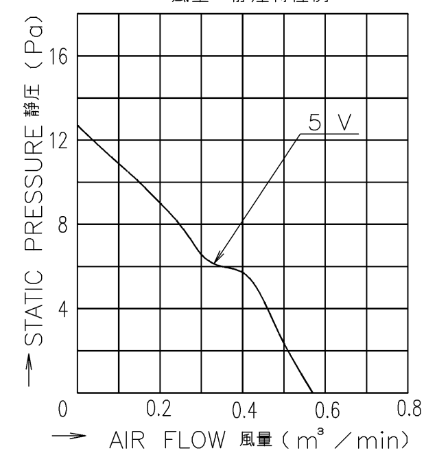
PERFORMANCE CURVES 風量-静圧特性例
