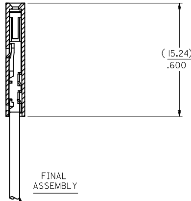
FINAL ASSEMBLY
