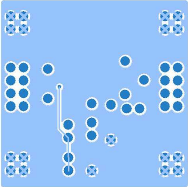
Figure 10. Typical Board Layout, Bottom Side
