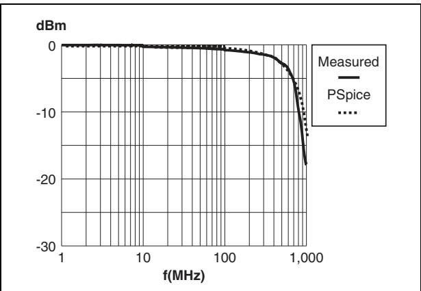
Figure 26. Attenuation comparison
