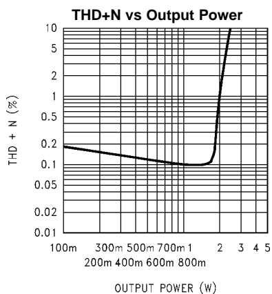
V_{DD} = 12V , R_L = 8\Omega , SE operation, A_V = 10 single channel driven/single channel measured, f_{IN} = 1kHz
