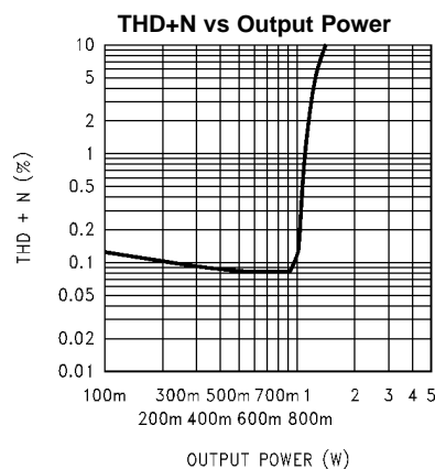
V_{DD} = 12V , R_L = 16\Omega , SE operation, A_V = 10 single channel driven/single channel measured, f_{IN} = 1kHz
