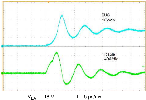
Figure 9-3. Disabled, 35-V, 1210, X7R C OUT Capacitor Without SMAJ18
