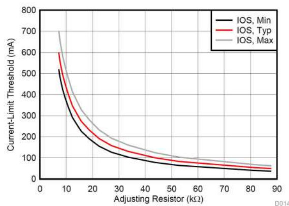
Figure 8-3. Current-Limit Setting vs Adjusting Resistor
