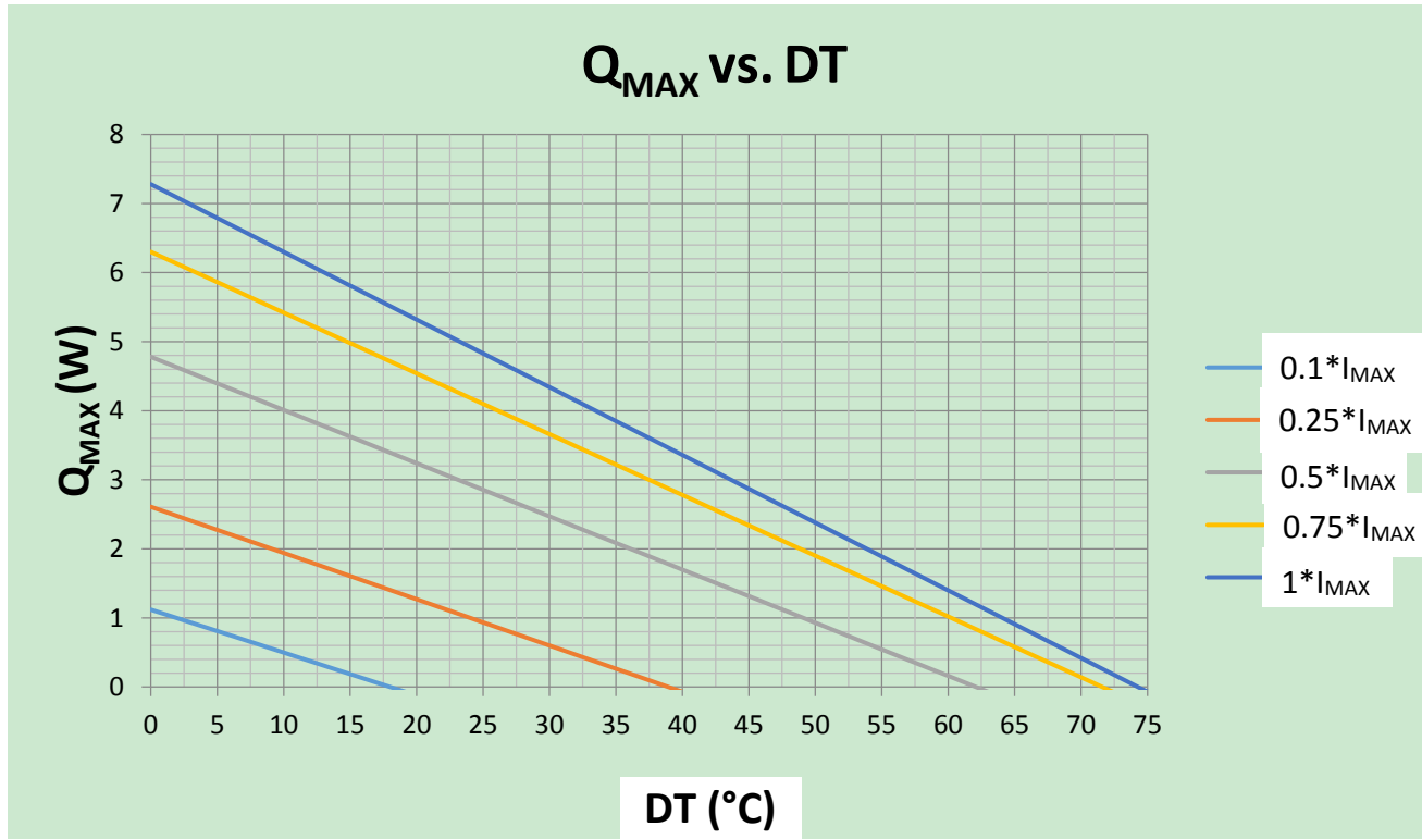
Figure 2. Q MAX vs. DT
