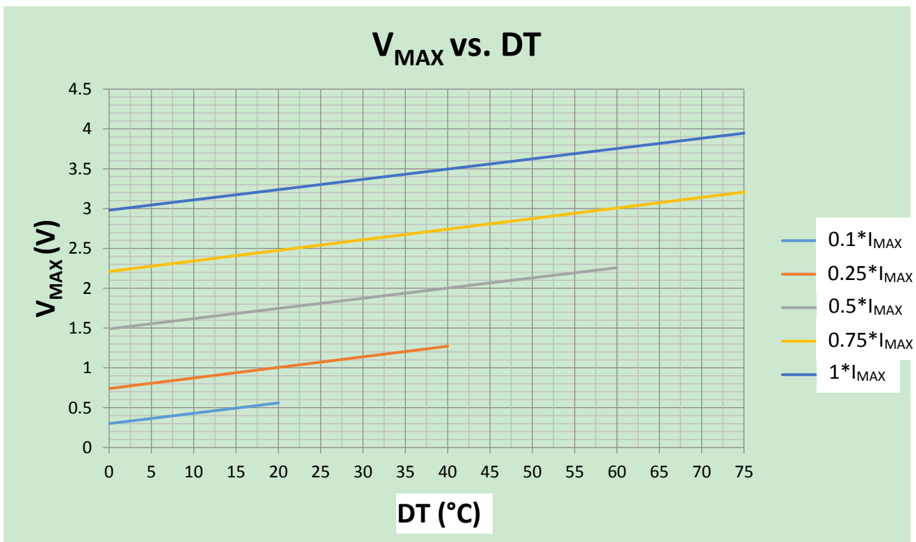
Figure 3. V MAX vs. DT
