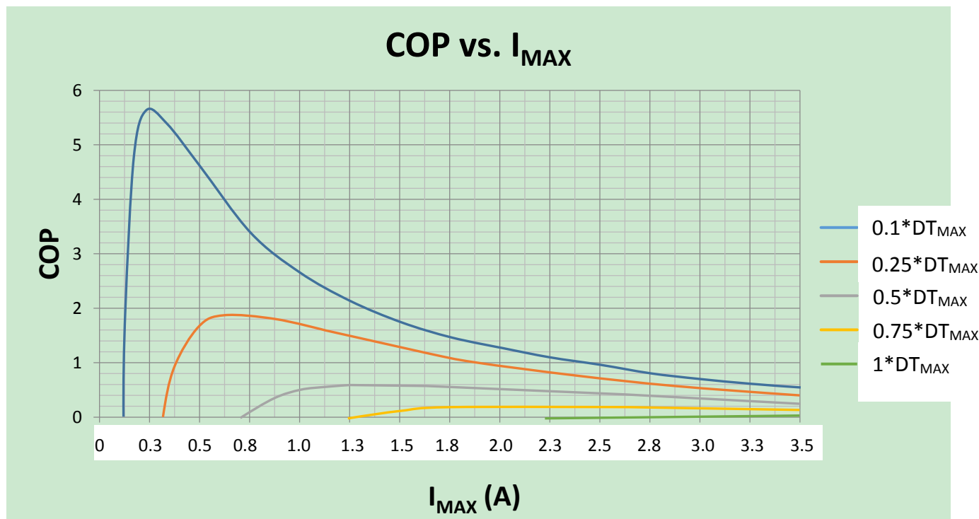
Figure 5. COP vs. I MAX
