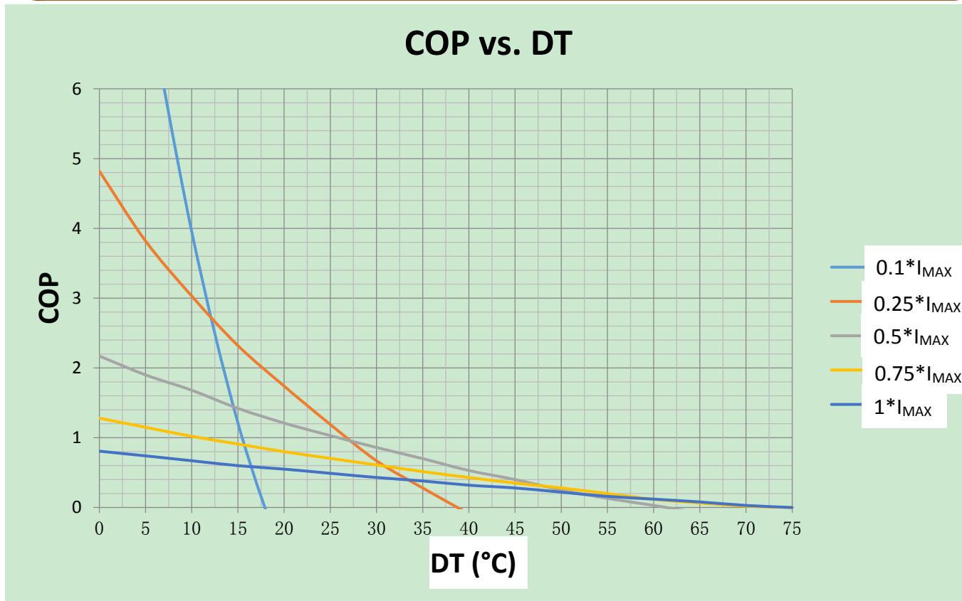
Figure 4. COP vs. DT
