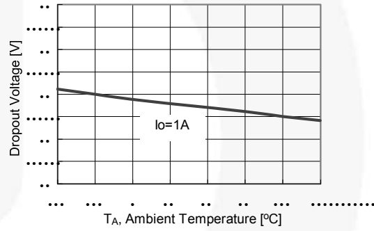
Figure 5. Dropout Voltage
