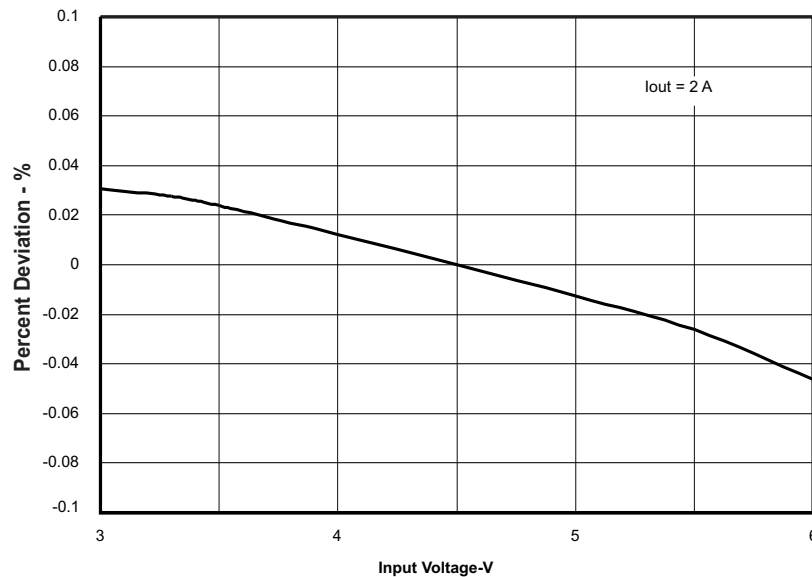
Figure 4. TPS54418EVM-375 Line Regulation
