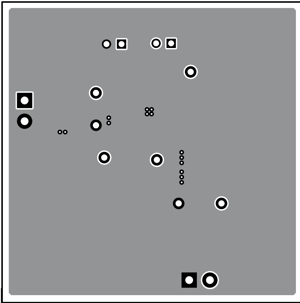
Figure 14. TPS54418EVM-375 Layout 3
