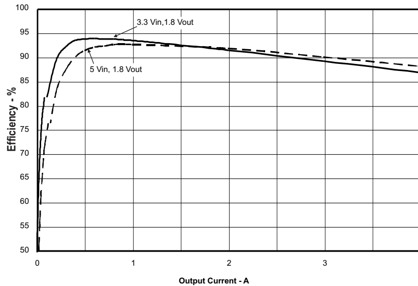
Figure 1. TPS54418EVM-375 Efficiency
