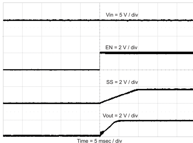
Figure 10. TPS54418EVM-375 Start-up Relative to Enable
