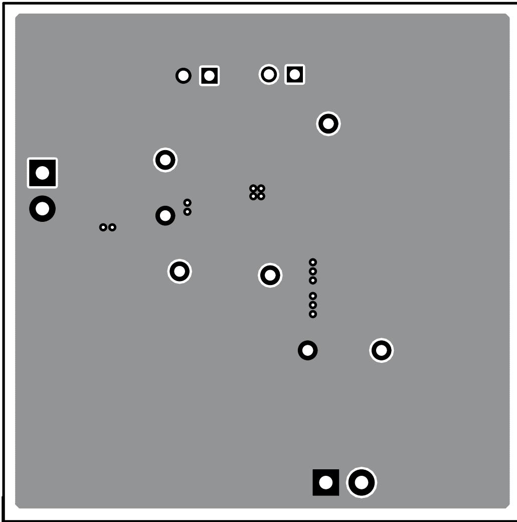
Figure 13. TPS54418EVM-375 Layout 2
