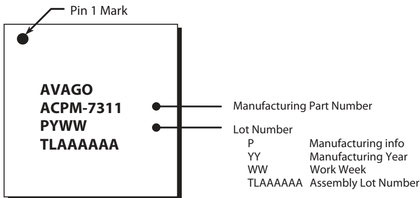
Figure 13. Marking Specifications
