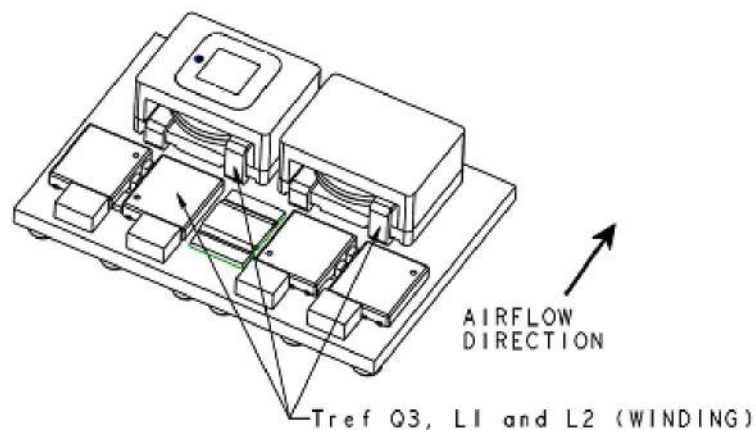
Preferred airflow direction and location of hot-spot of the module ( T_{ref} ).
