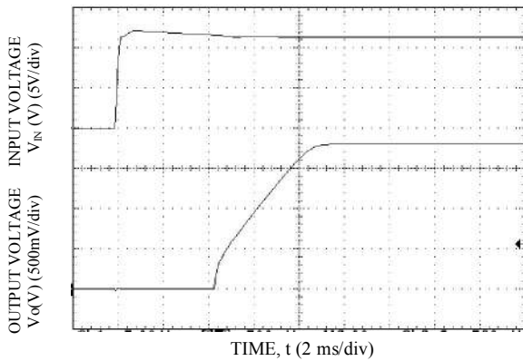
Start-up Using Input Voltage ( V_{IN} = 12V , I_o = I_{o,max} ), V_o = 1.8V , T_a = 25^\circ C
