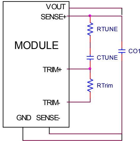
Circuit diagram showing connection of R_{TUNE} and C_{TUNE} to tune the control loop of the module
