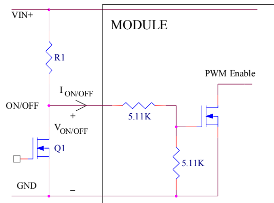
Remote On/Off Implementation using ON/OFF
