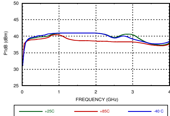
Input P1dB vs. Temperature @ Vdd = +5V
