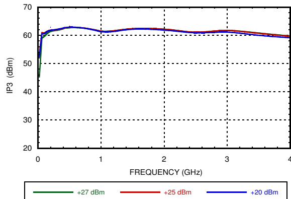
Input IP3 vs. Tone Power @ Vdd = +5V
