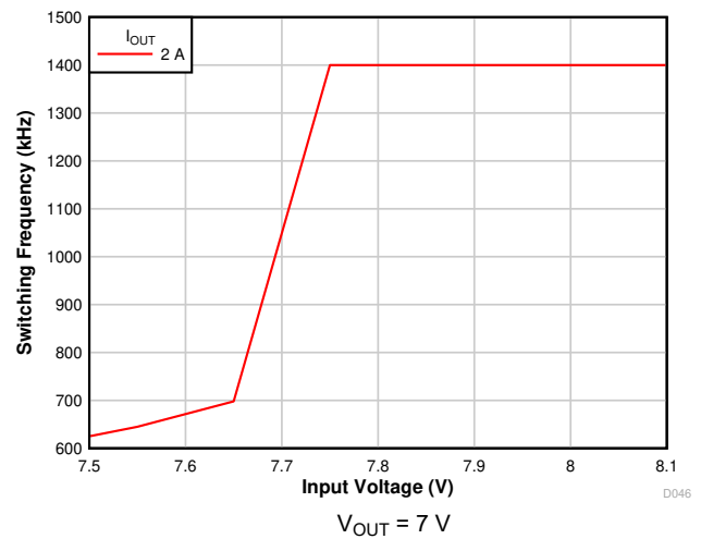
Figure 7-12. Frequency Foldback
