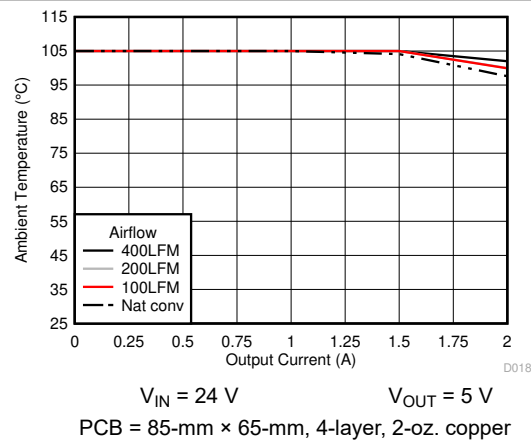
Figure 6-16. Safe Operating Area
