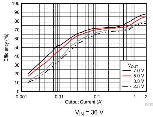
Figure 6-18. Efficiency versus Output Current
