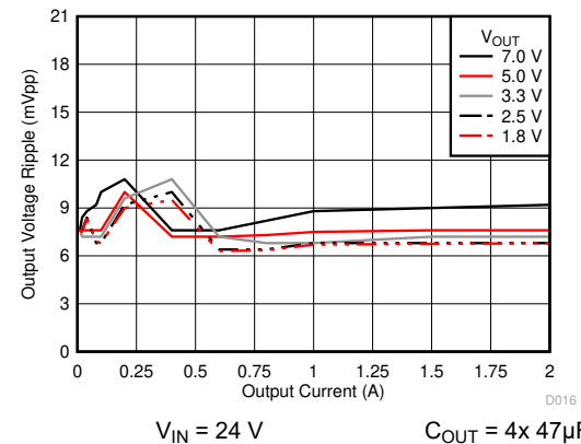
Figure 6-14. Voltage Ripple versus Output Current
