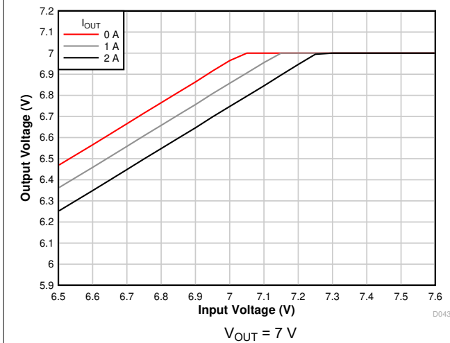
Figure 7-11. Voltage Dropout
