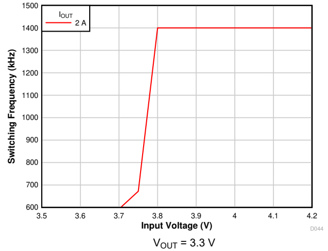
Figure 7-8. Frequency Foldback
