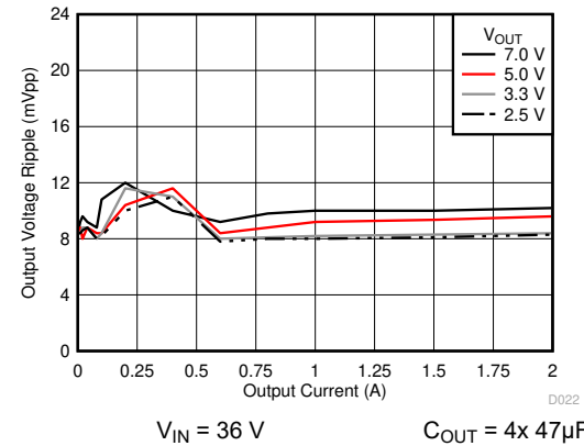
Figure 6-20. Voltage Ripple versus Output Current
