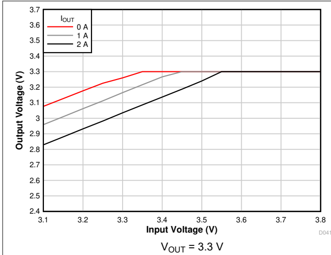
Figure 7-7. Voltage Dropout
