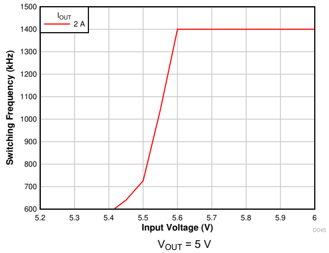
Figure 7-10. Frequency Foldback
