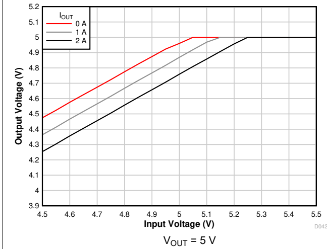
Figure 7-9. Voltage Dropout
