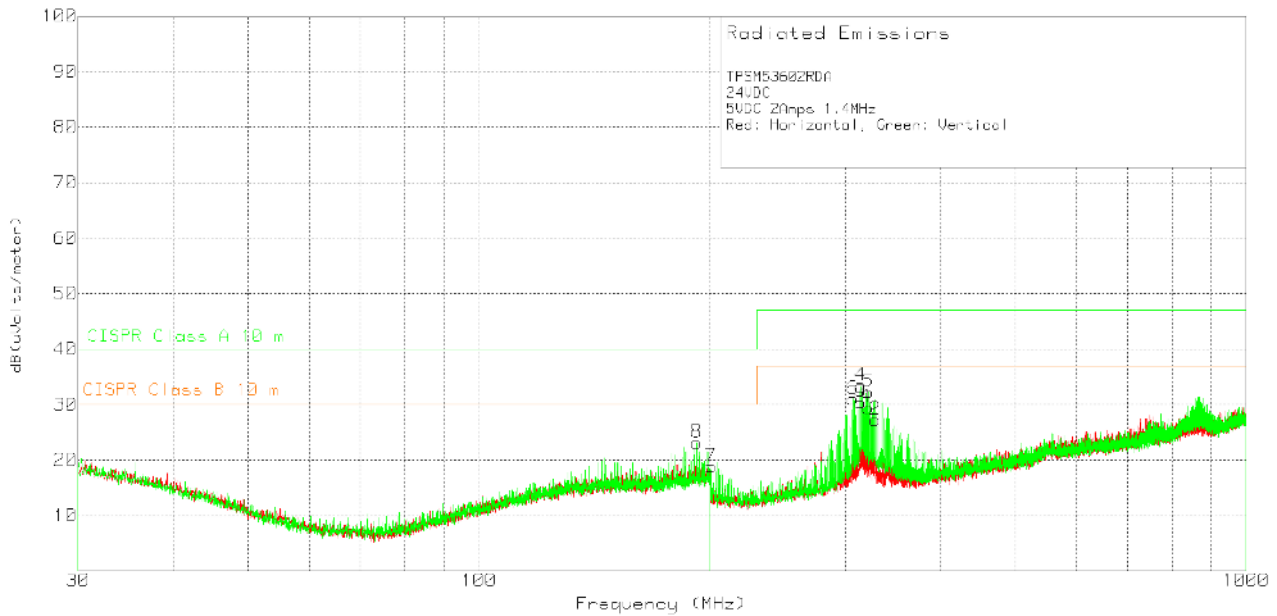
Figure 10-5. Radiated Emissions 24-V Input, 5-V Output, 2-A Load
