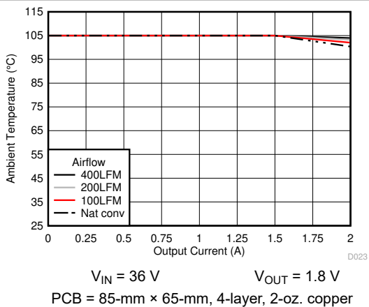
Figure 6-21. Safe Operating Area
