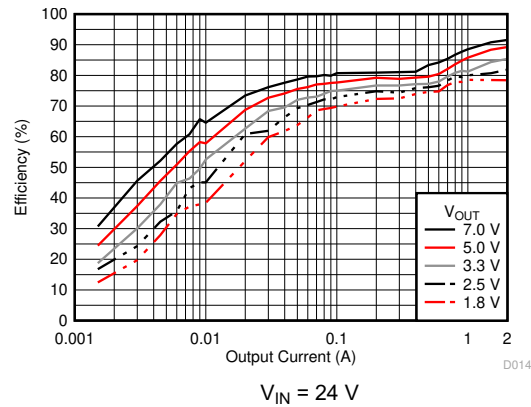
Figure 6-12. Efficiency versus Output Current
