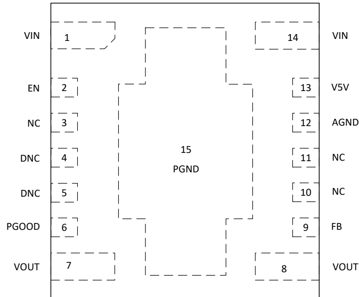
Figure 5-1. RDA Package 15-Pin QFN Top View
