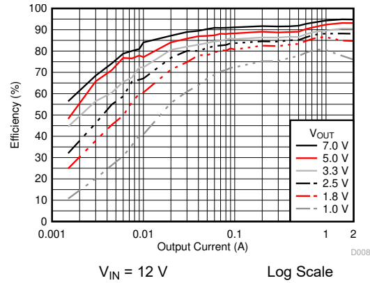
Figure 6-7. Efficiency versus Output Current
