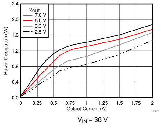
Figure 6-19. Power Dissipation versus Output Current
