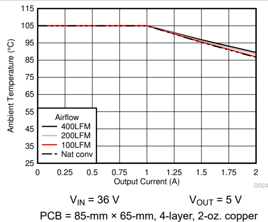
Figure 6-22. Safe Operating Area
