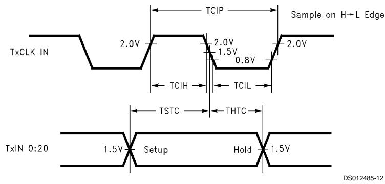
FIGURE 7. DS90CF561 (Transmitter) Setup/Hold and High/Low Times
