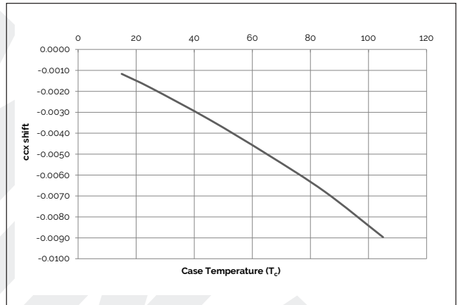
Figure 13: Typical DC ccx Shift vs. Case Temperature 4
