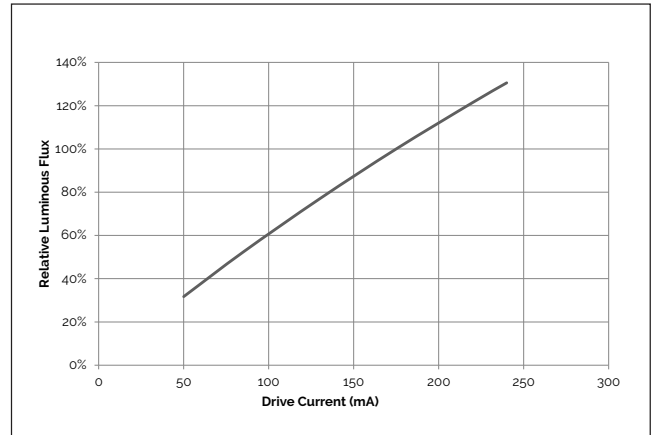
Figure 11: Typical Relative Flux vs. Current 1,2
