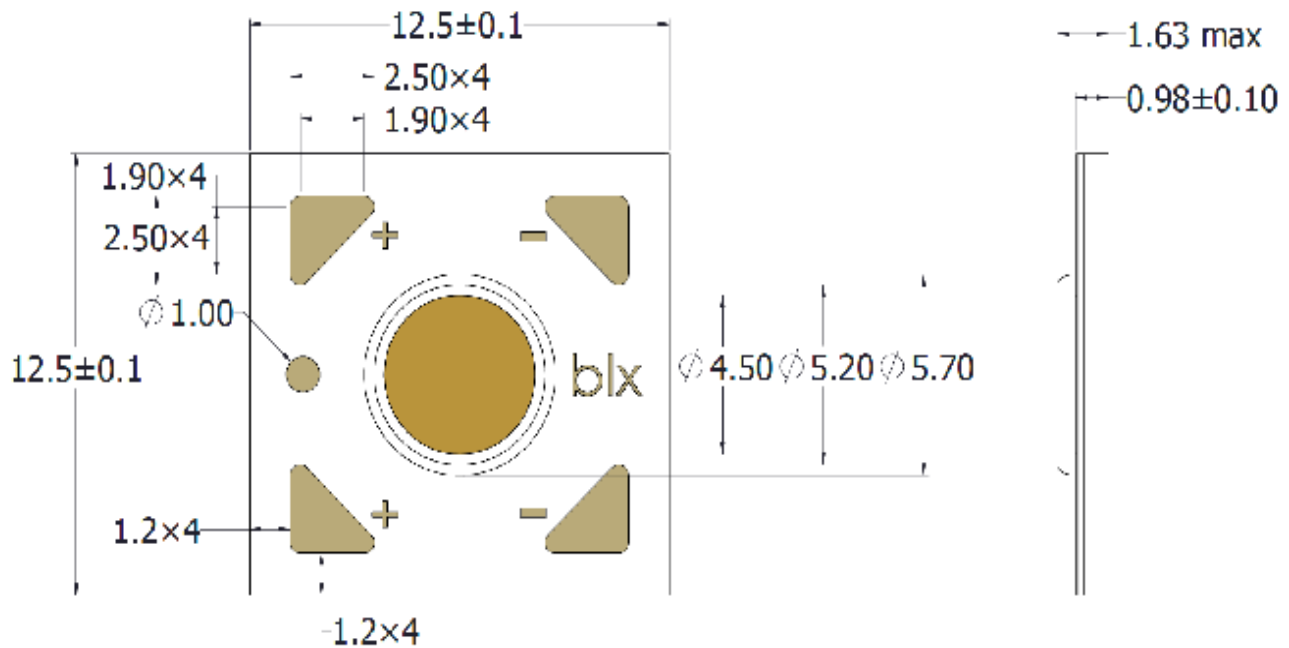
Figure 17: Drawing for V4 HD LED Array
