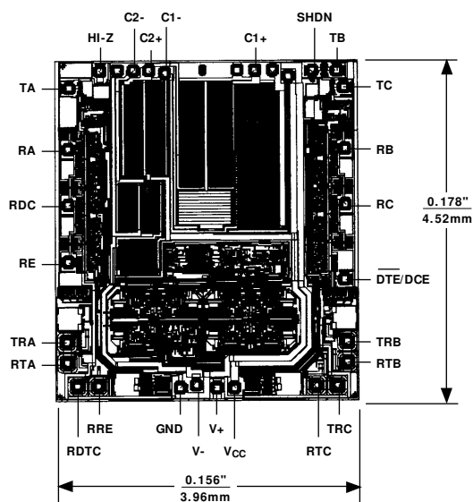
Chip Topography
