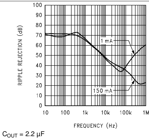
Figure 13. Ripple Rejection
