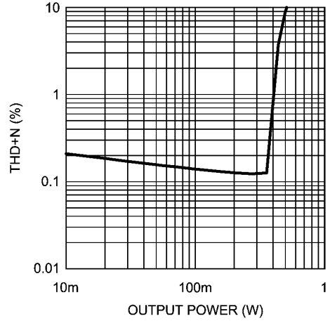
THD+N+N vs Output Power V_{DD} = 3V, R_L = 8\Omega, \text{ and } f = 1\text{kHz}
