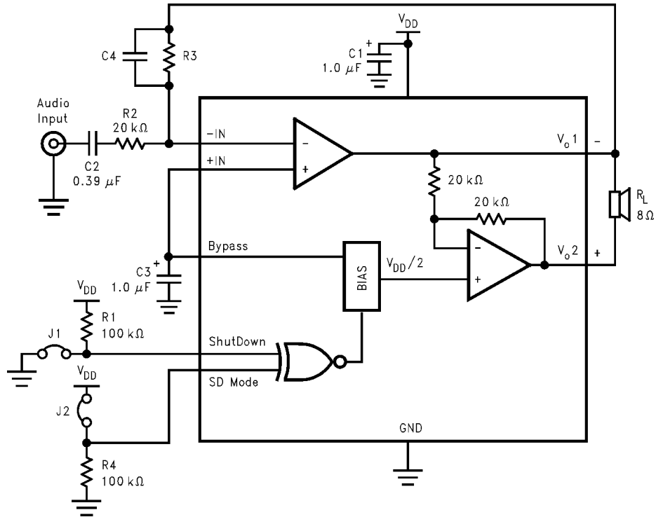
FIGURE 3. HIGHER GAIN AUDIO AMPLIFIER
